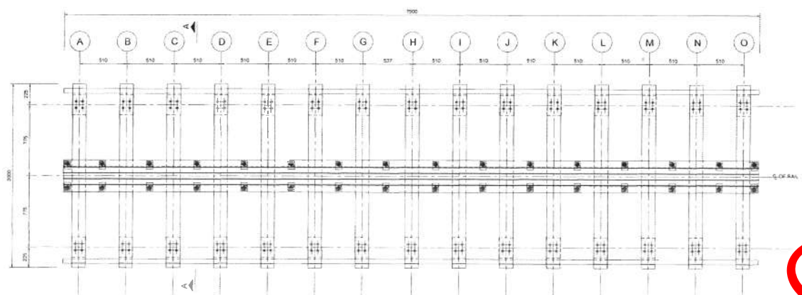
PLAN VIEW OF BRIDGE
