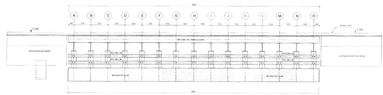
ELEVATION OF BRIDGE
