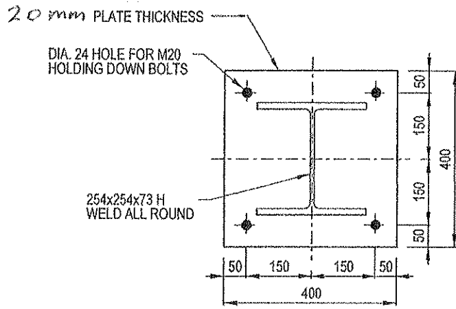
PLAN (6m Column & Base Plate)
