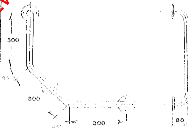
DOG LEG SIDE RAIL REF. DL2, WITHOUT CENTRE FLANGE REF. DL3, WITH CENTRE FLANGE
