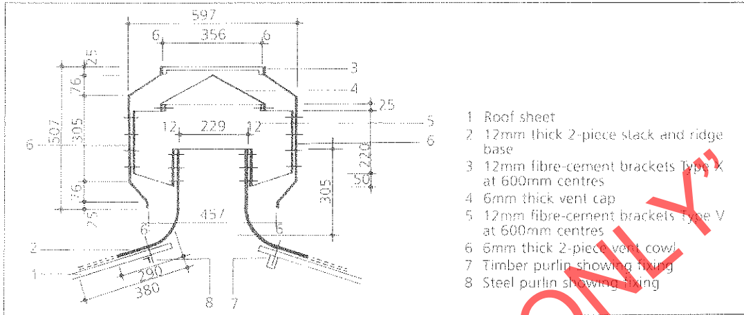
FIG. 4 DIMENSIONS OF VENTILATOR
