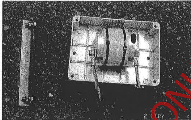
Figure 7. The internal view of the enclosure and the mounting bracket.
