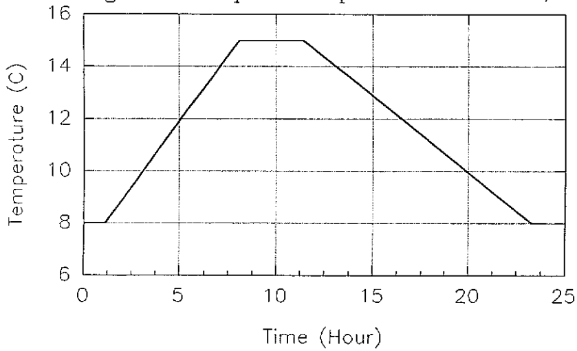
Fig 5.2.1 Temperature profile – Grades A,B
