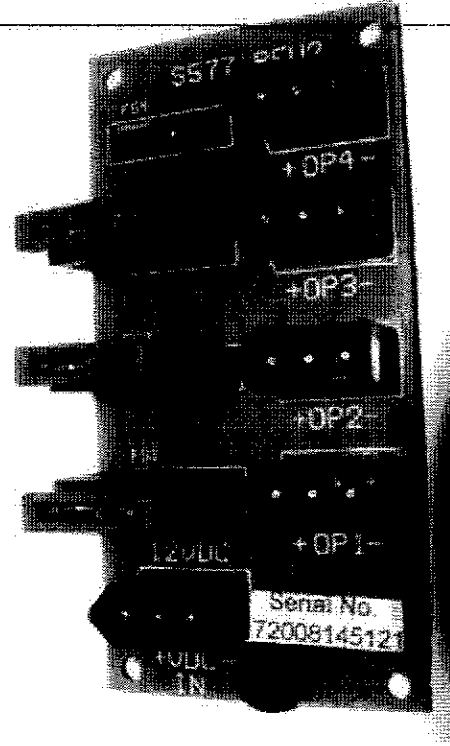
Fuse board SOS type S577
