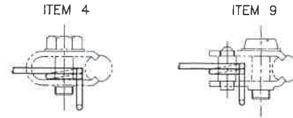
DETAIL VIEW OF CONTACT WIRE CLIPS (SCALE 1:1)
