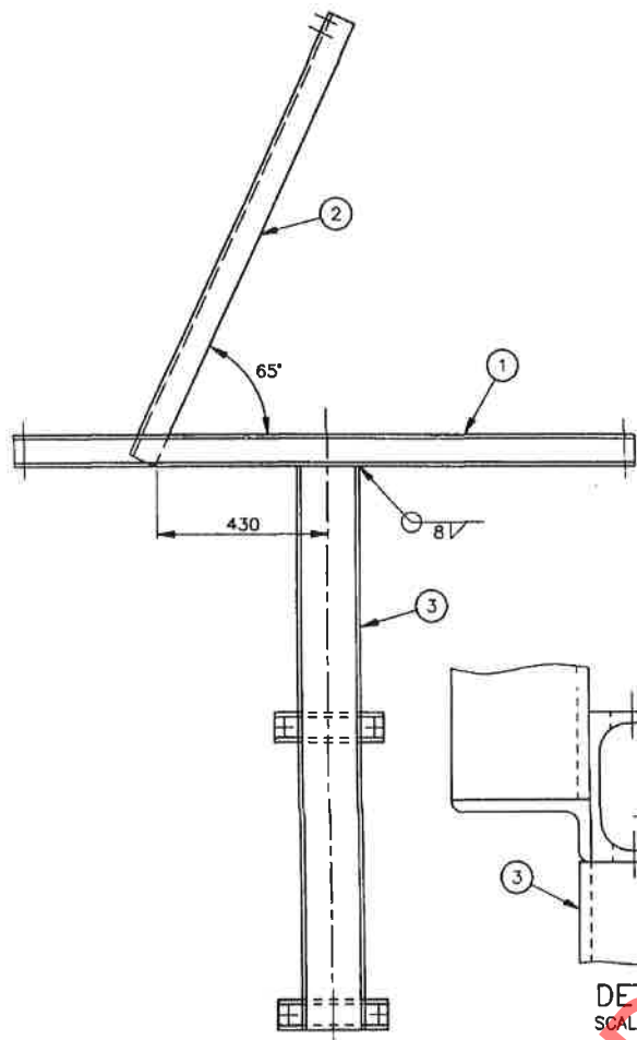
CONCRETE MAST ARRANGEMENT
