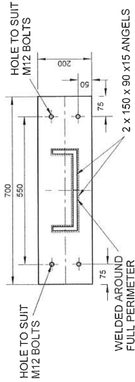
BASE PLATE ( 700mm x 200mm x 20mm )
