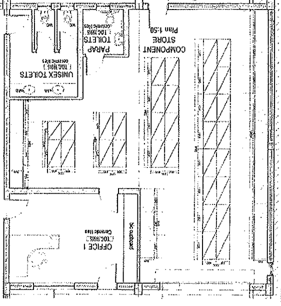
TOOL STORE Plan 1:50
