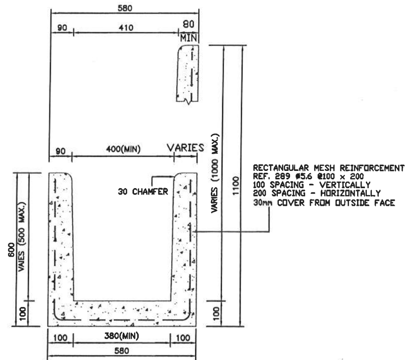
TYPICAL SECTION SCALE 1:10
