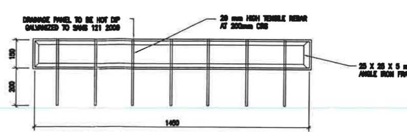
DETAIL OF DRAINAGE PANEL 1:10
