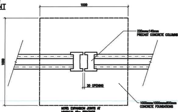
DETAIL OF EXPANSION JOINT 1:10
