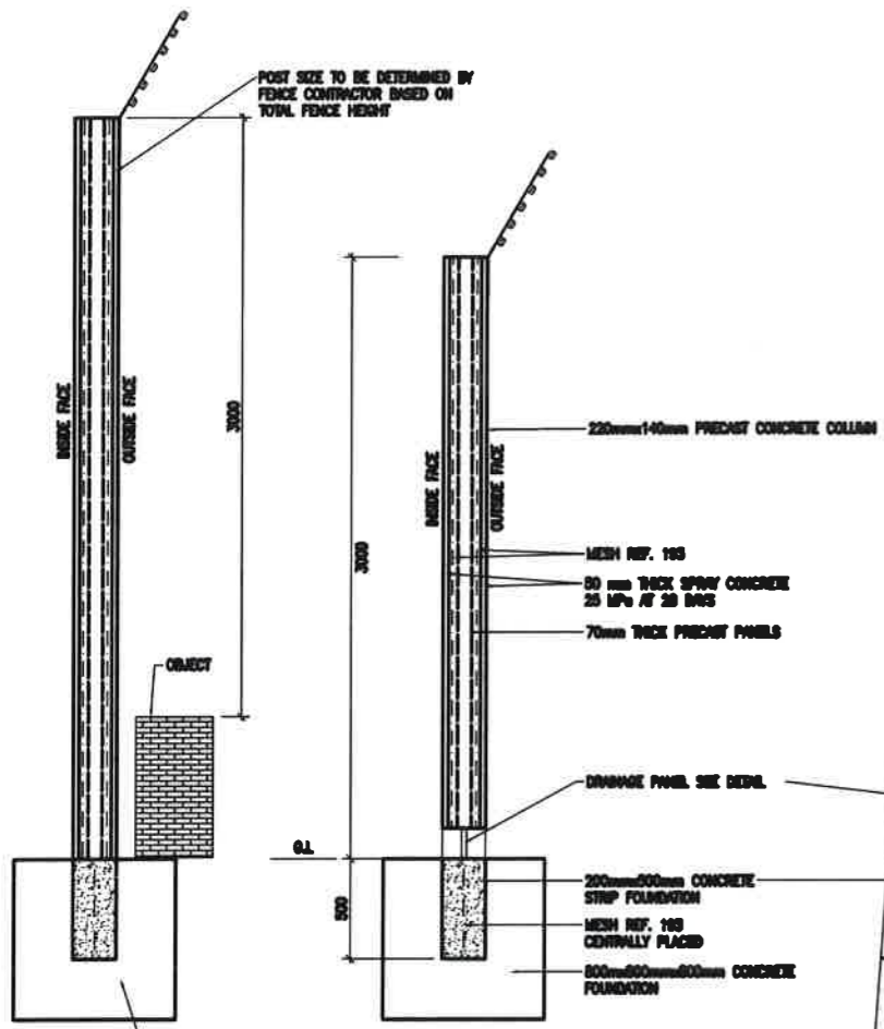
TYPICAL SECTION AT DRAINAGE PANEL 1:20
