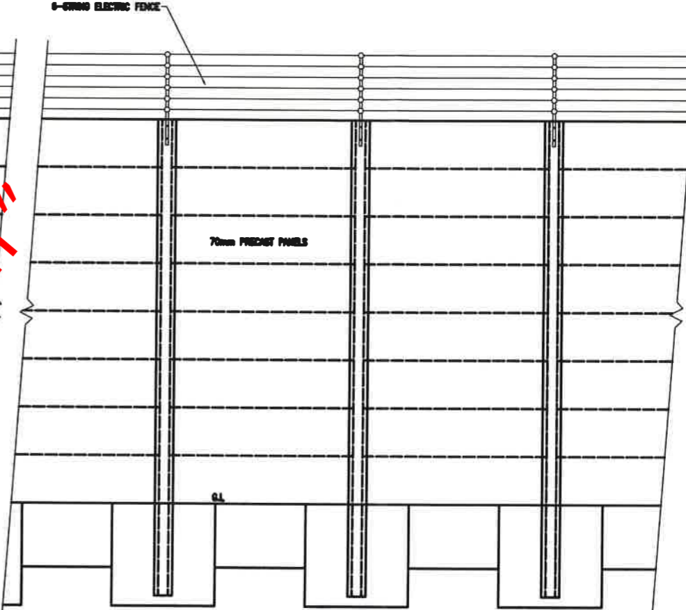
STANDARD PANEL ELEVATION
